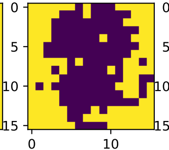
T = 2.5
