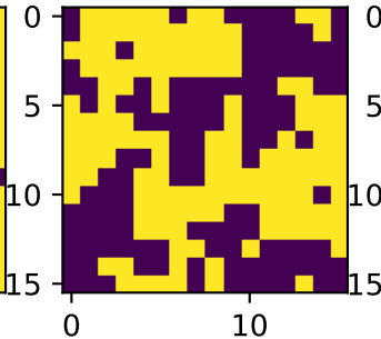
T = 3.5
