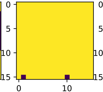
T = 1.5
