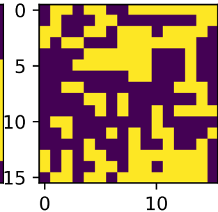
T = 5.0
